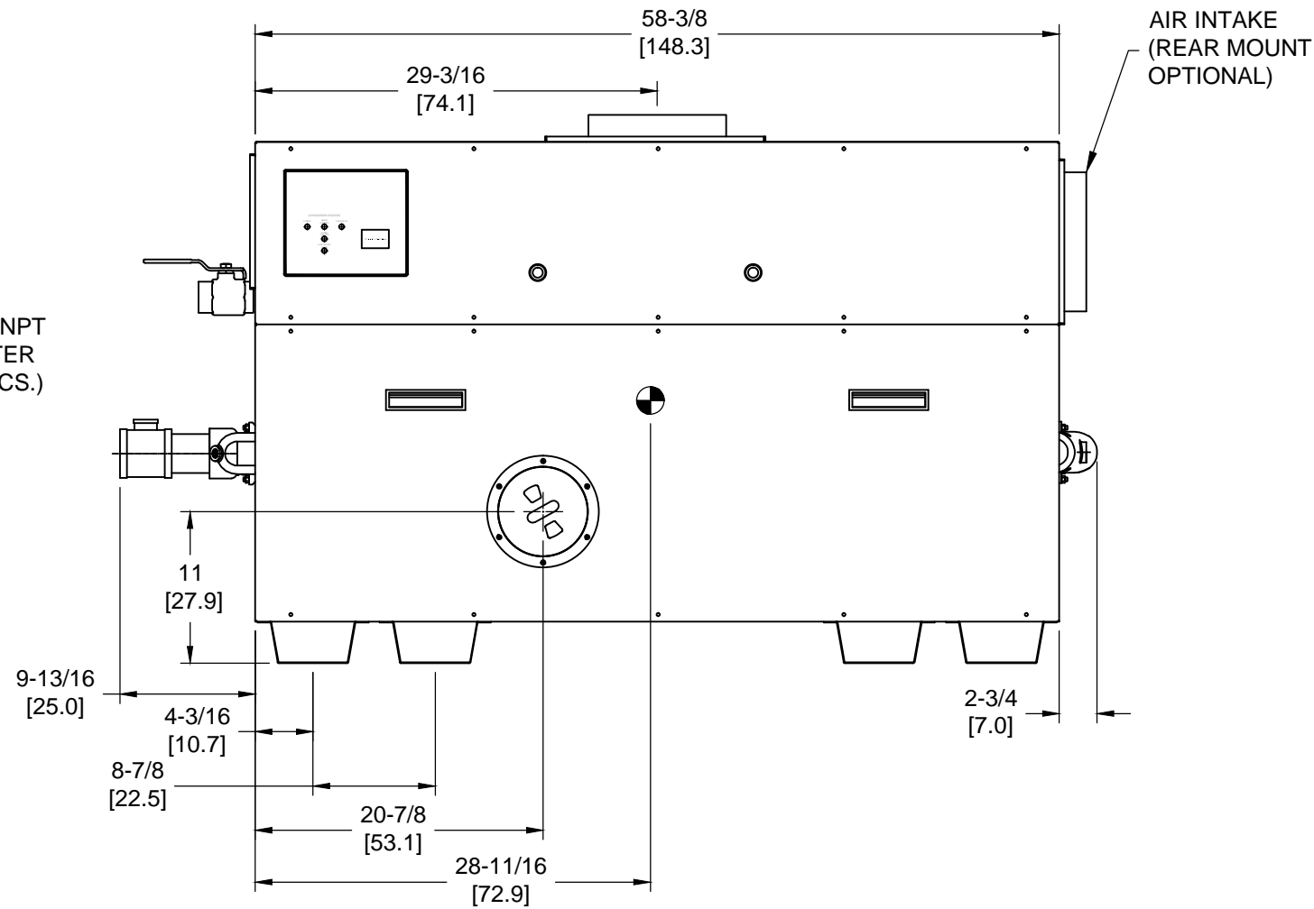
FRONT VIEW
